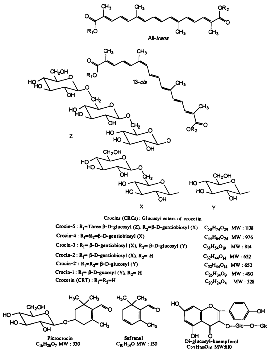
Fig. 1. Structures of saffron components. MW = Molecular mass.
