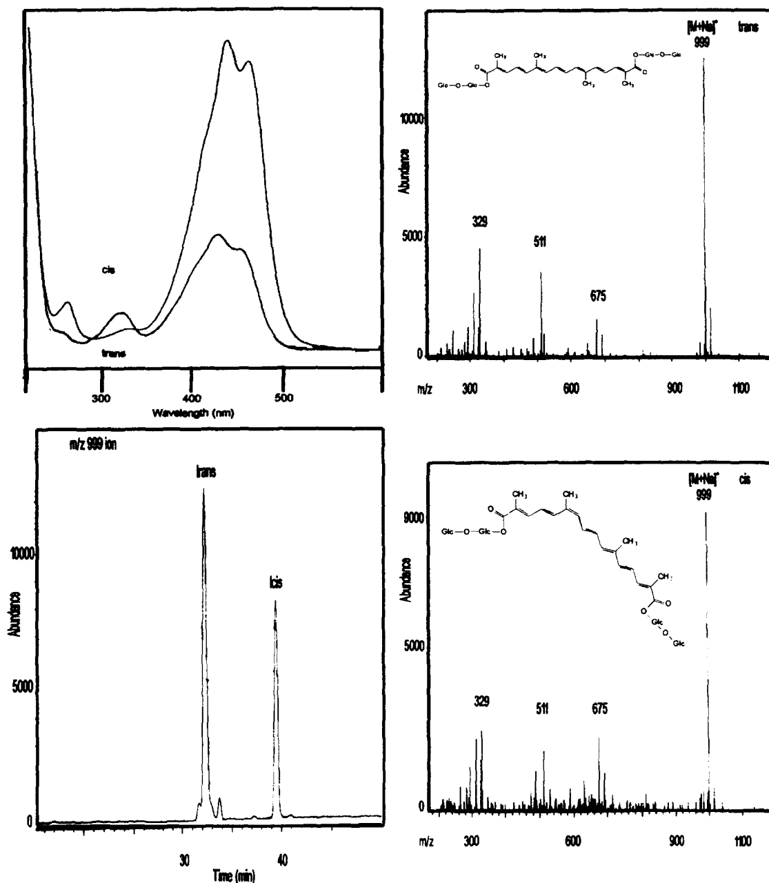
Fig. 6. Mass spectra, UV-visible spectra and selected-ion chromatogram of cis - and trans -crocins-4 [crocin di( \beta -D-gentiobiosyl)ester].
