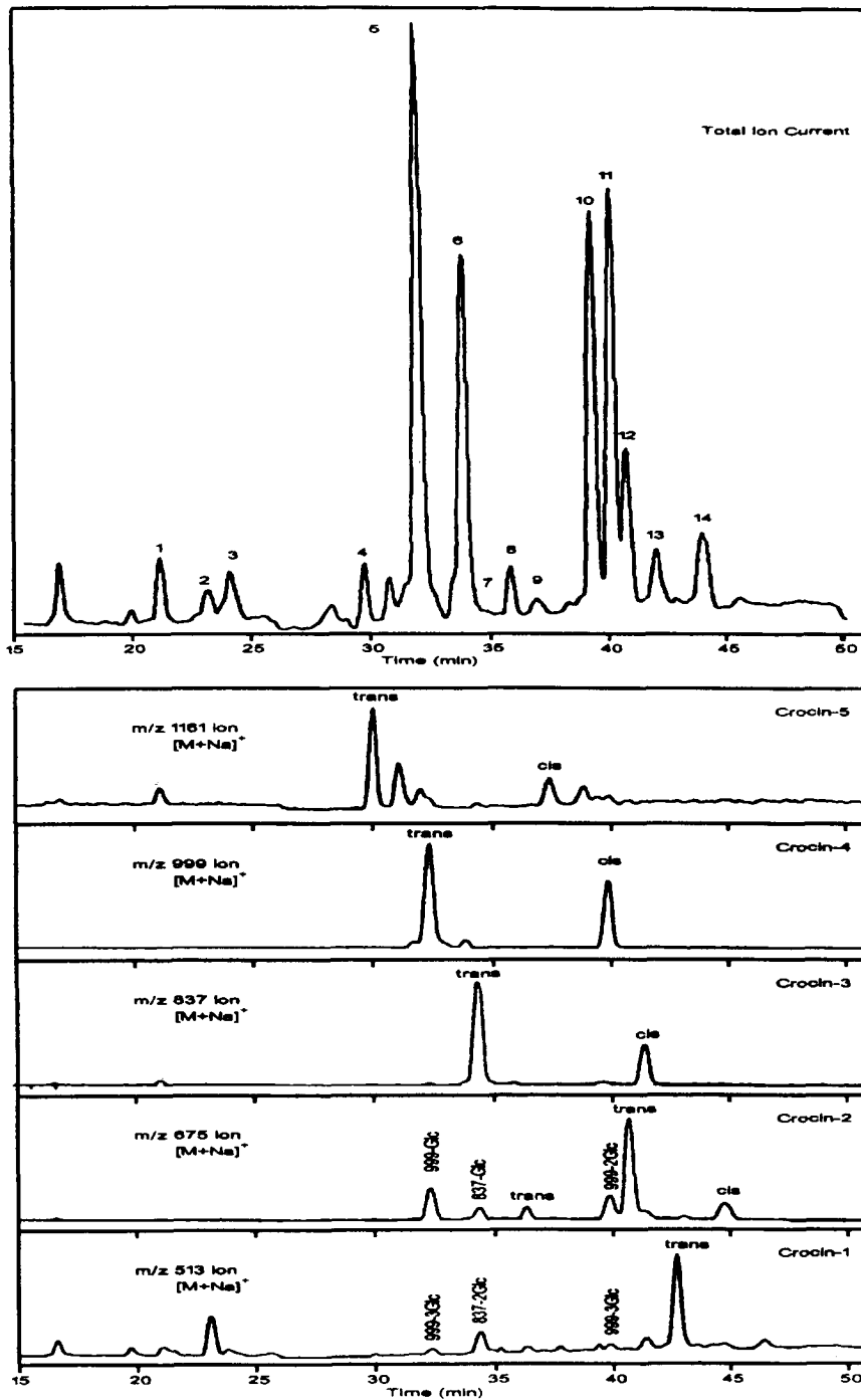
Fig. 3. Total ion chromatogram and selected-ion chromatograms for the HPLC-ES-MS analysis of a methanol-water (50:50) extract of saffron.
